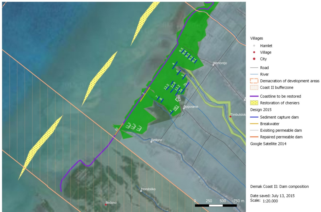
Figure 5.5. Spatial design of coastal safety measures in Coast I/II planned for 2015, in collaboration with MMAF.
