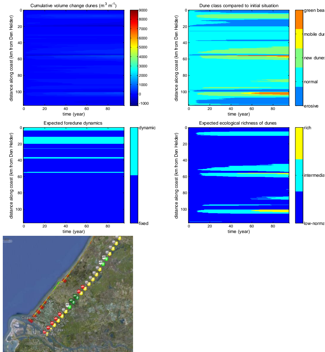
Figure 3. Dune development related to scenario 1: 'Autonomous development with SLR ( 2 \text{ mm y}^{-1} )'. The horizontal axis represents time in years, and the vertical axis distance along the coast running from north to south. The upper part of each plot therefore represents the development of the North-Holland coast and the lower part the South-Holland coast. Upper left: cumulative dune volume change (i.e. dune volume with respect to starting situation). Upper right: dune classes. Middle left: expected foredune dynamics. Middle right: expected biodiversity based on the dune classes. Lower left: corresponding screen shot of the ITHK visualised in Google Earth at t = 100 y for this scenario.
