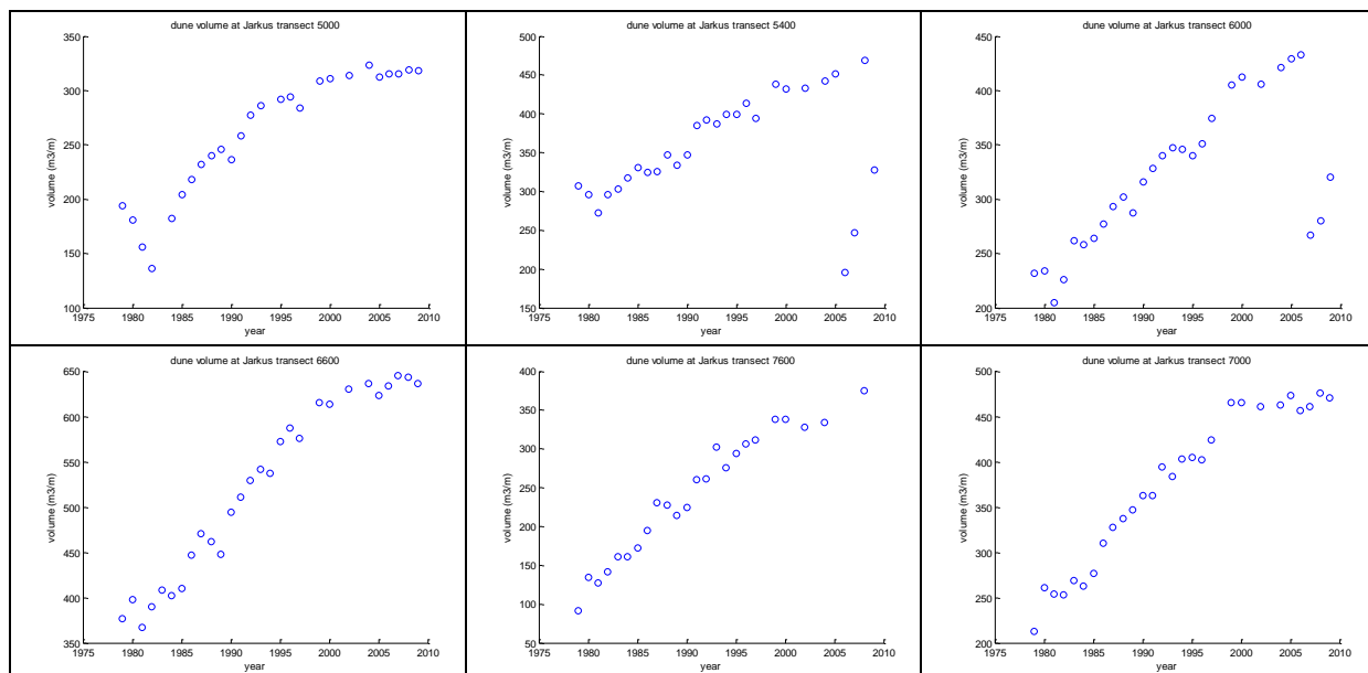
Figure A 2. Examples of dune volumes at Schiermonnikoog, at the location where new dune development from around 2000 on resulted in a green beach. NB: the landward reference varies between transects. Therefore only trends can be compared and not absolute volumes.
