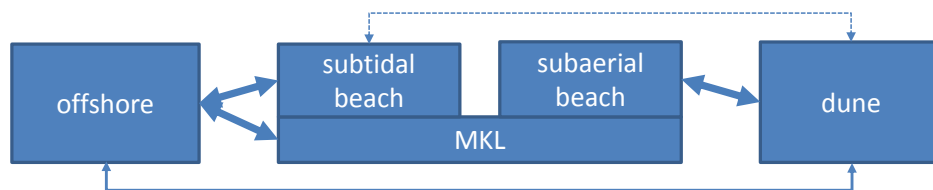
Figure 1. Correlations between volume changes of different parts of the active profile, based on analyses by Sierd de Vries. All correlations are positive, and the thickness of the arrows indicates the strength of the correlations. Dune is the volume > +3 NAP, subaerial beach between +3 m NAP and MLW, subtidal between MLW and the +3 m NAP mirrored in MLW, and offshore lower than that. MKL is the sum of the two parts of the beach, i.e. the standard Dutch measure for beach sand volume.
