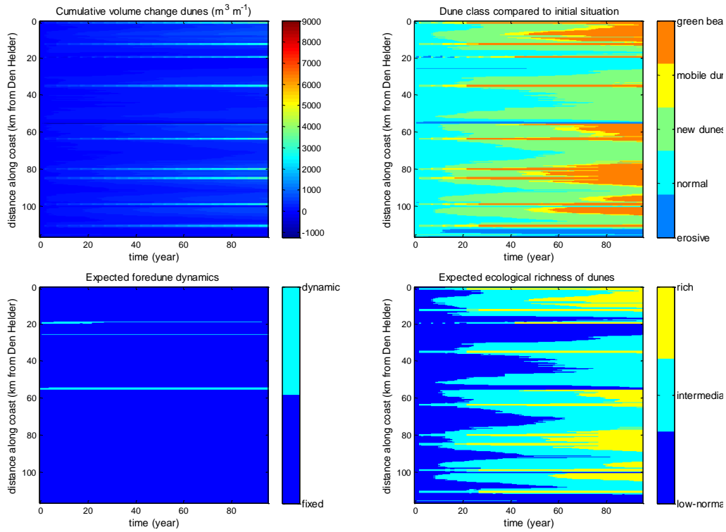
Figure 5. Dune development related to scenario 3: 'Minimal consolidation 5-year intervals with SLR'. Panels are the same as in Figure 3.
