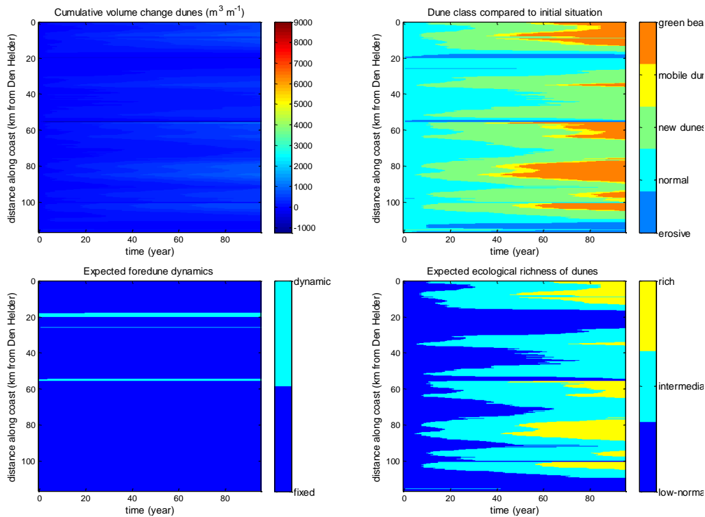
Figure 4. Dune development related to scenario 2: 'Minimal consolidation with SLR'. Panels are the same as in Figure 3. Note that the scales in the upper left panels vary between pictures.
