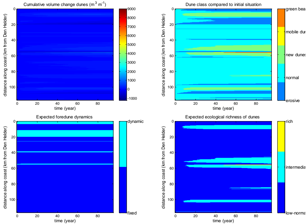
Figure 7. Dune development related to scenario 5: 'Revetments with SLR'. Panels are the same as in Figure 3.
