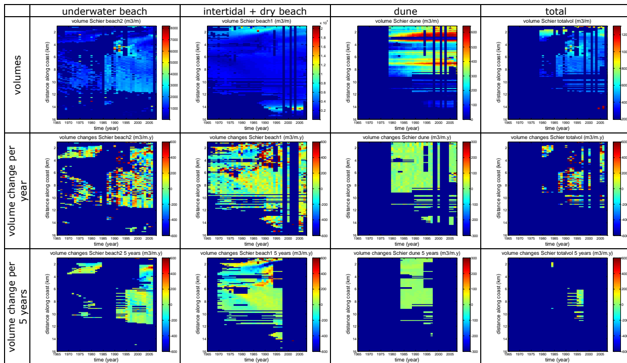
Figure A 1. Example of trends in volumes on Schiermonnikoog. Vertical axis: distance along shoreline, horizontal axis: time. Dark blue indicates no data. Volumes (upper panels) can only be compared within one transect location.
