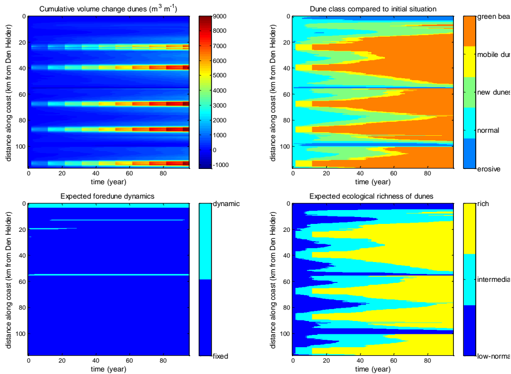
Figure 6. Dune development related to scenario 4: 'Seaward with sand engines with SLR'. Panels are the same as in Figure 3.
